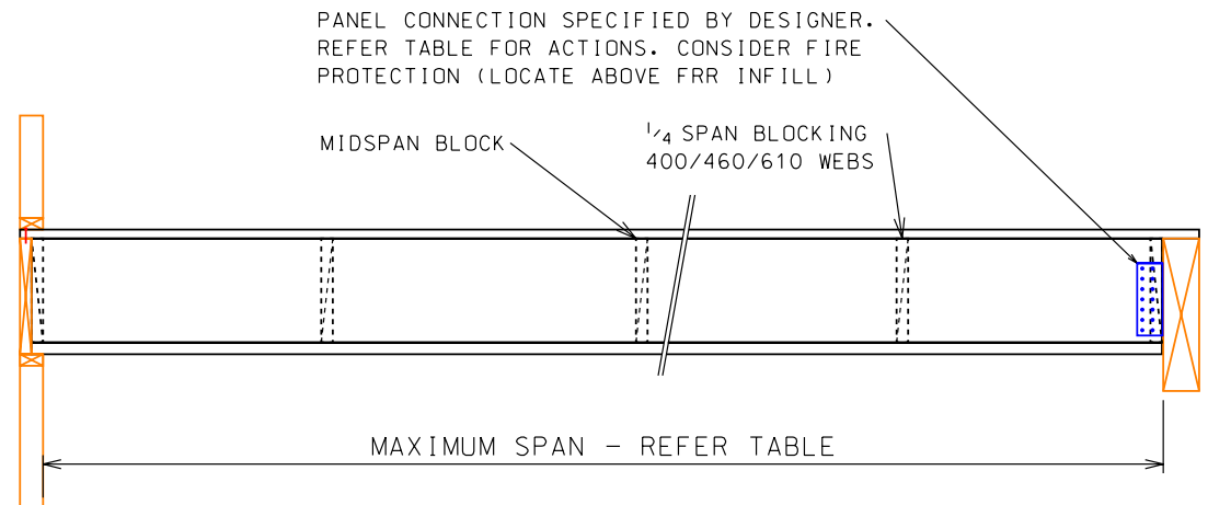
PANEL LONG SECTION SCALE 1:20
