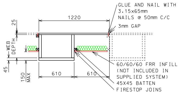
TYPICAL PANEL SECTION SCALE 1:20
